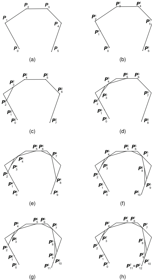
Fig. 4 A sample graph of degree elevation on control polygon (a) can be interpreted as corner cutting after inserting knots t_0^0 (b), t_2^0 (c), t_3^0 (d), t_4^0 (e), t_6^0 (f), t_7^0 (g), and t_8^0 (h) one by one
